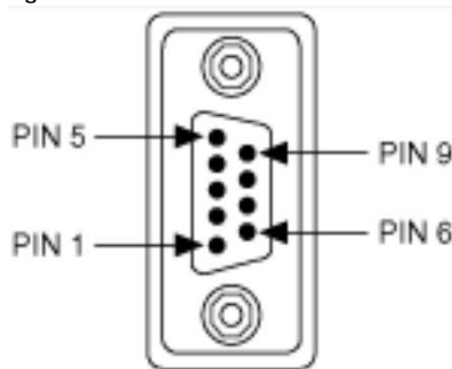
Figure 49 DB-9 Connector Pins
