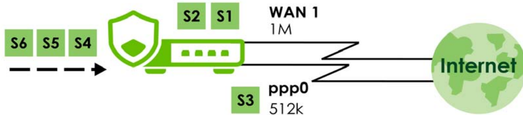
Figure 109 Weighted Round Robin Algorithm Example
