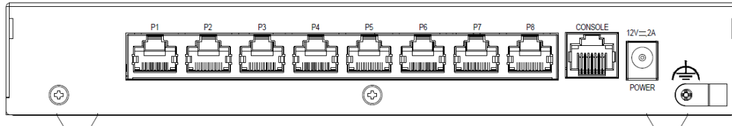
Figure 43 USG FLEX 100HP Rear Panel
