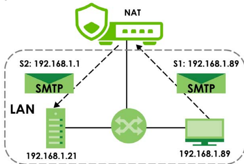
Figure 122 LAN to LAN Traffic
