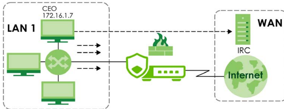
Figure 171 Limited LAN to WAN IRC Traffic Example
