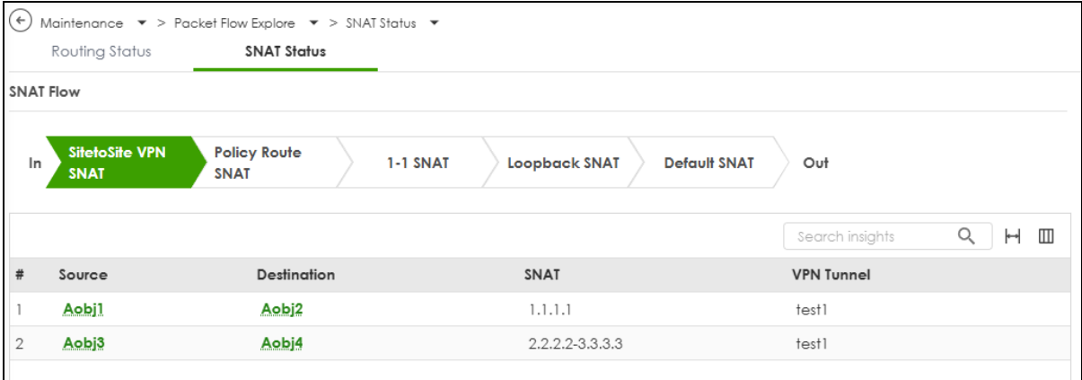
Figure 318 Maintenance > Packet Flow Explore > SNAT Status (SitetoSite VPN SNAT)
