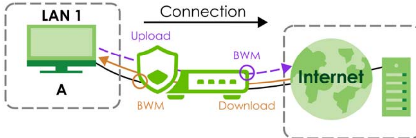
Figure 126 LAN1 to WAN Connection and Packet Directions
