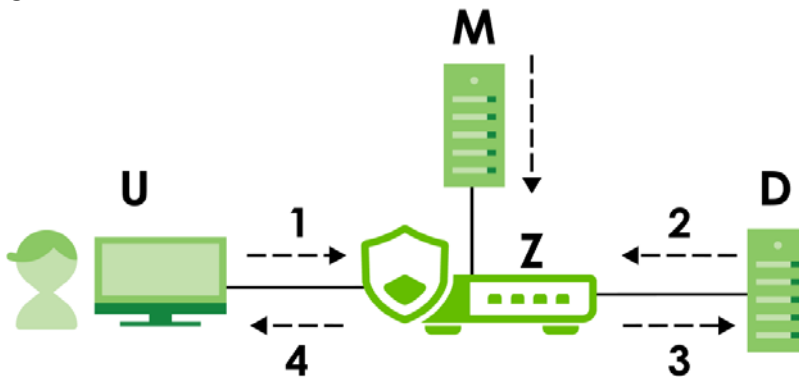
Figure 236 SSL Inspection Certificate Update Overview
