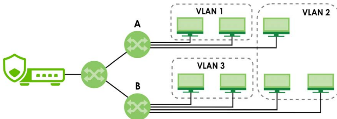
Figure 96 Example: After VLAN
