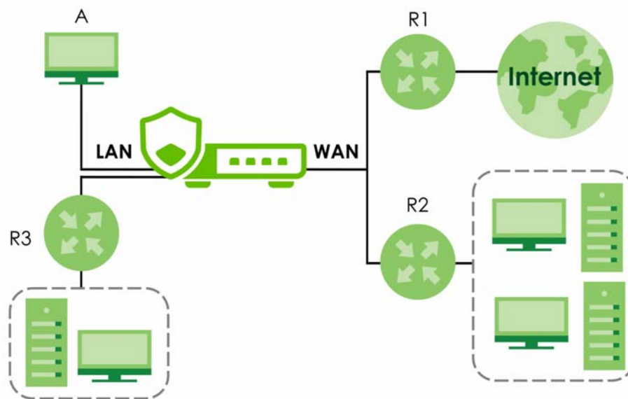
Figure 115 Example of Policy Routing Topology
