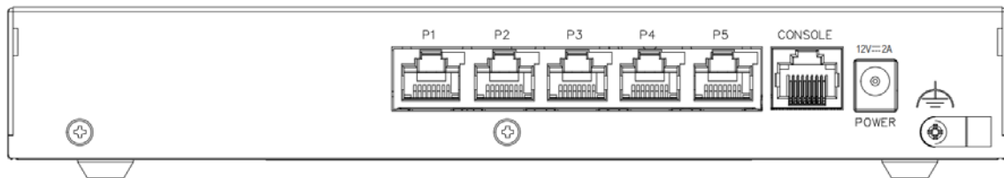
Figure 41 USG FLEX 50HP Rear Panel
