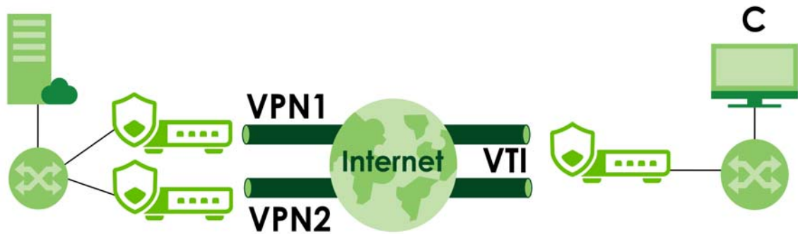
Figure 106 VTI and Trunk for VPN Load Balancing
