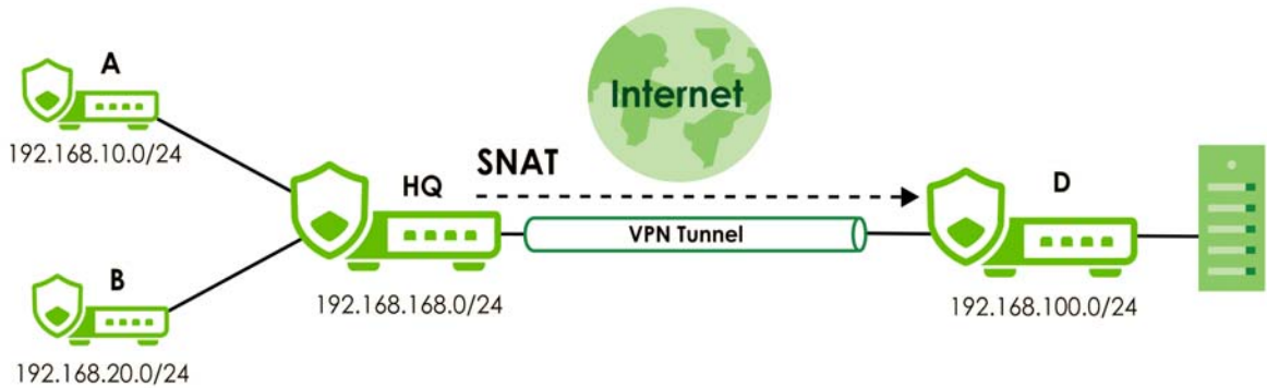
Figure 151 Policy Based VPN - SNAT Example Scenario
