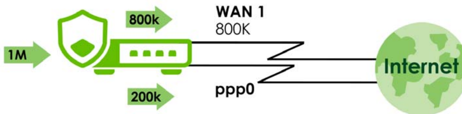
Figure 110 Spillover Algorithm Example
