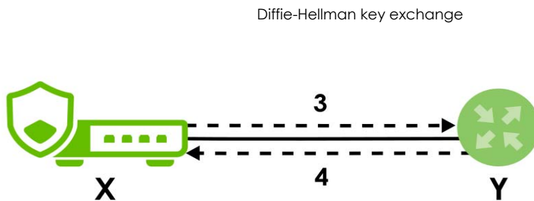
Figure 138 IKE SA: Main Negotiation Mode, Steps 3 - 4: DH Key Exchange
