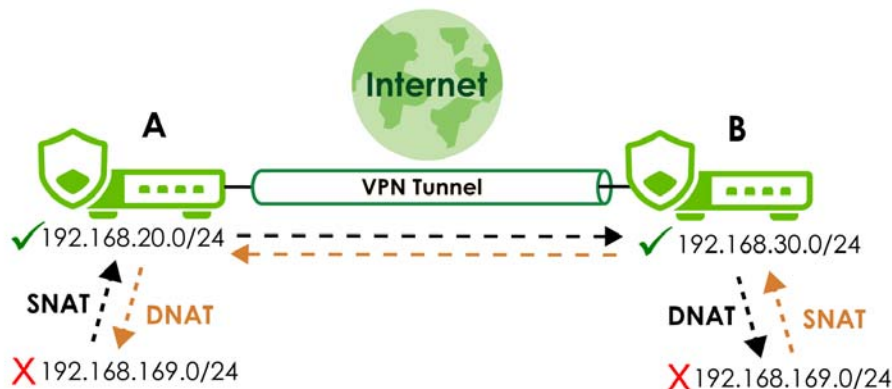
Figure 152 Policy Based VPN - 1:1 NAT Example Scenario
