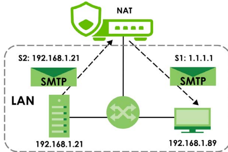
Figure 123 LAN to LAN Return Traffic
