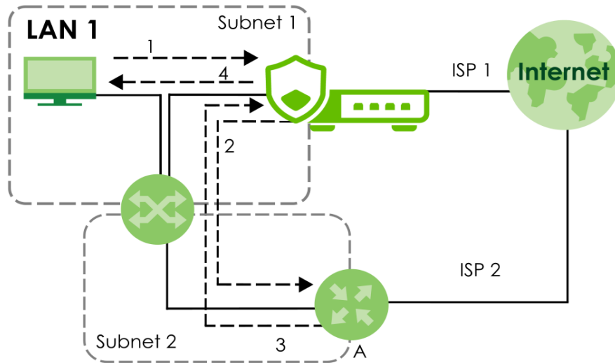
Figure 159 Using Virtual Interfaces to Avoid Asymmetrical Routes
