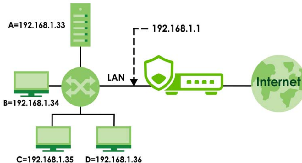
Figure 120 Multiple Servers Behind NAT Example
