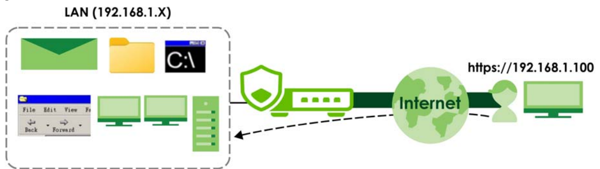
Figure 155 Network Access Mode: Full Tunnel Mode
