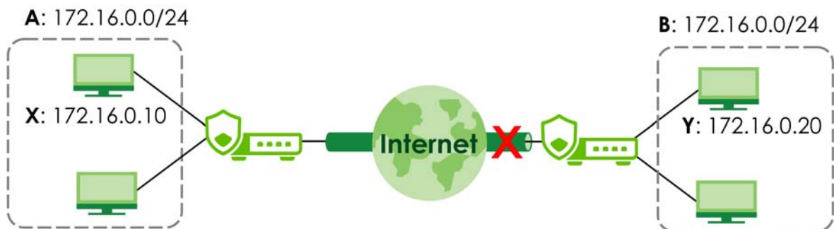
Figure 29 IP Address Conflict Causing VPN Failure
